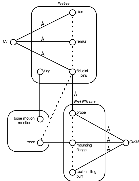
Figure 2. Registration graph of ISS RoboDoc system, showing induced links and event tags.
